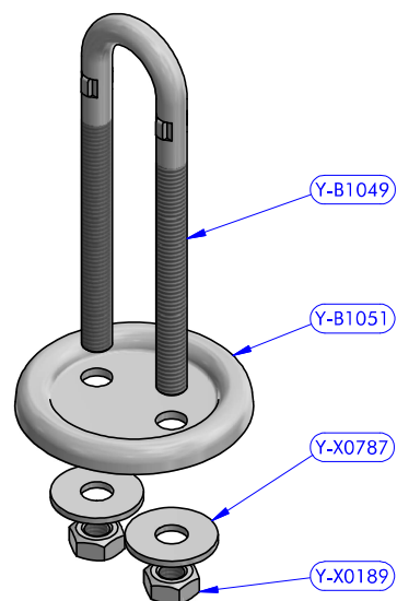
U-BOLT MOD. 7105
