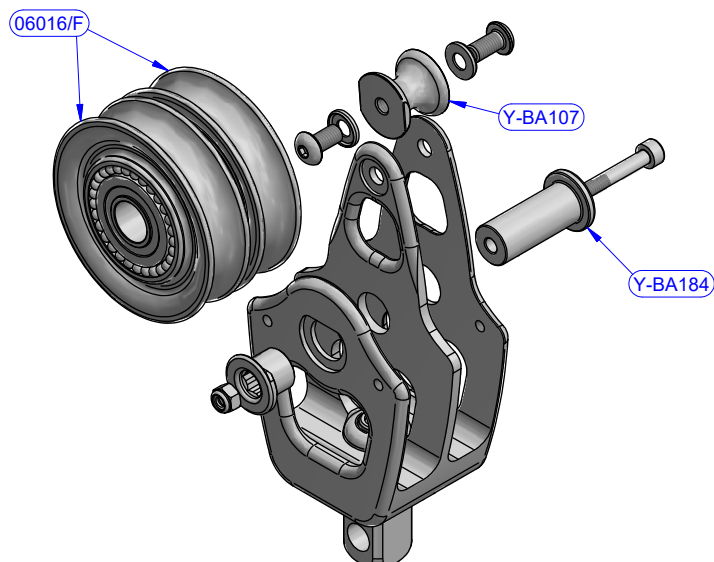
Double block Y-BA117
