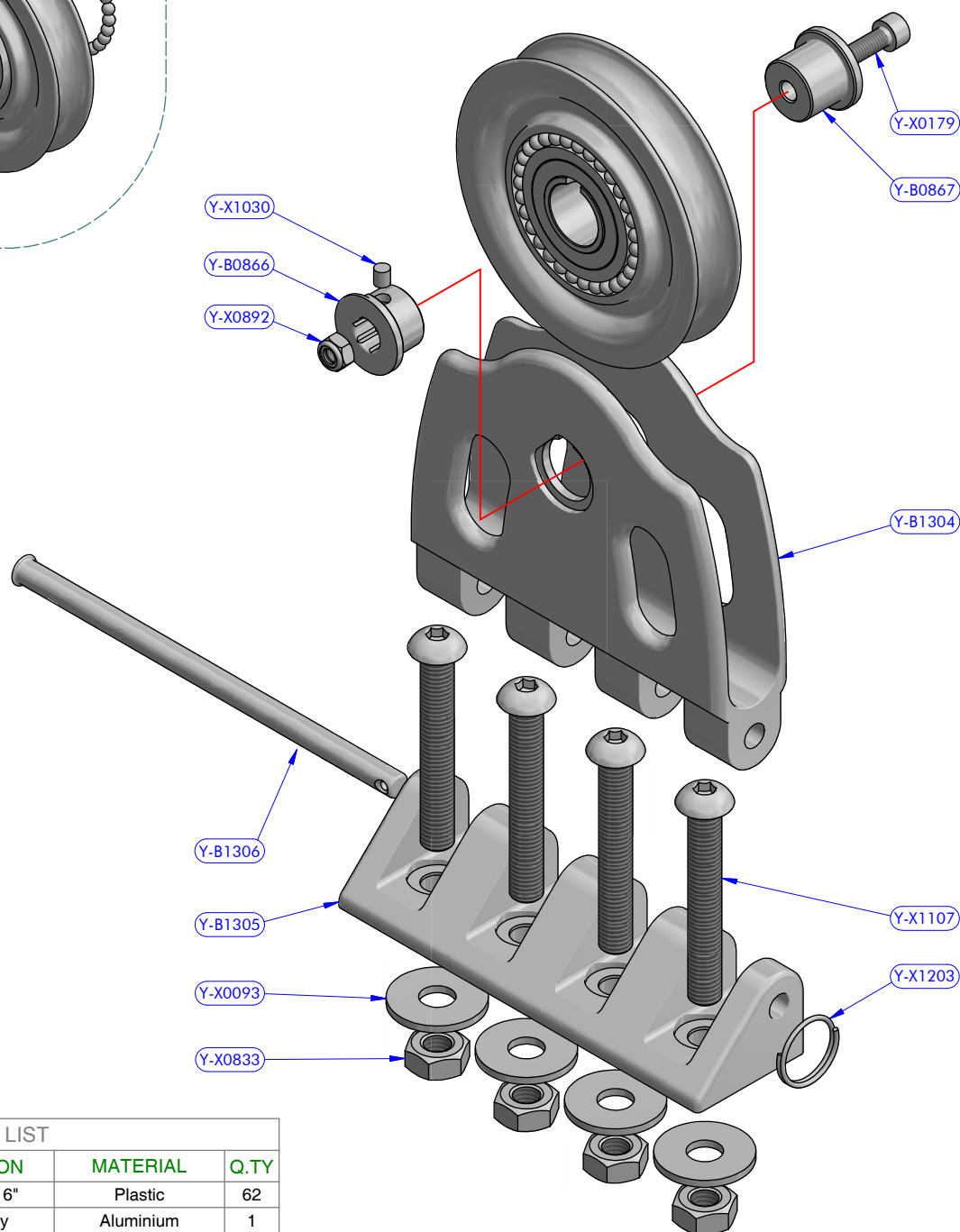
Sheave mod. 10021/A
