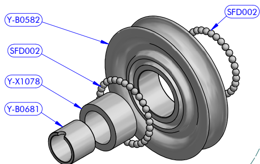
Sheave mod. 10021/A
