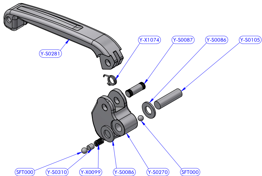
Cod.Y-SA072 Lever assy QR12
