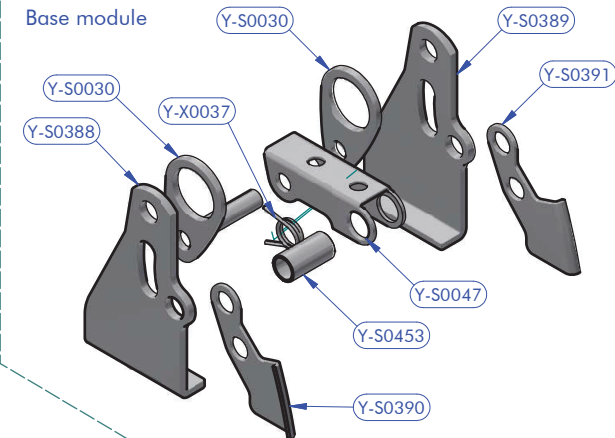
Cod.Y-SA046 Lever assy
