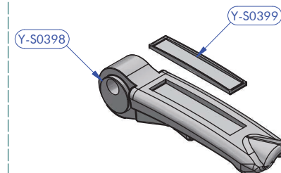
Cod.Y-SA046 Lever assy
