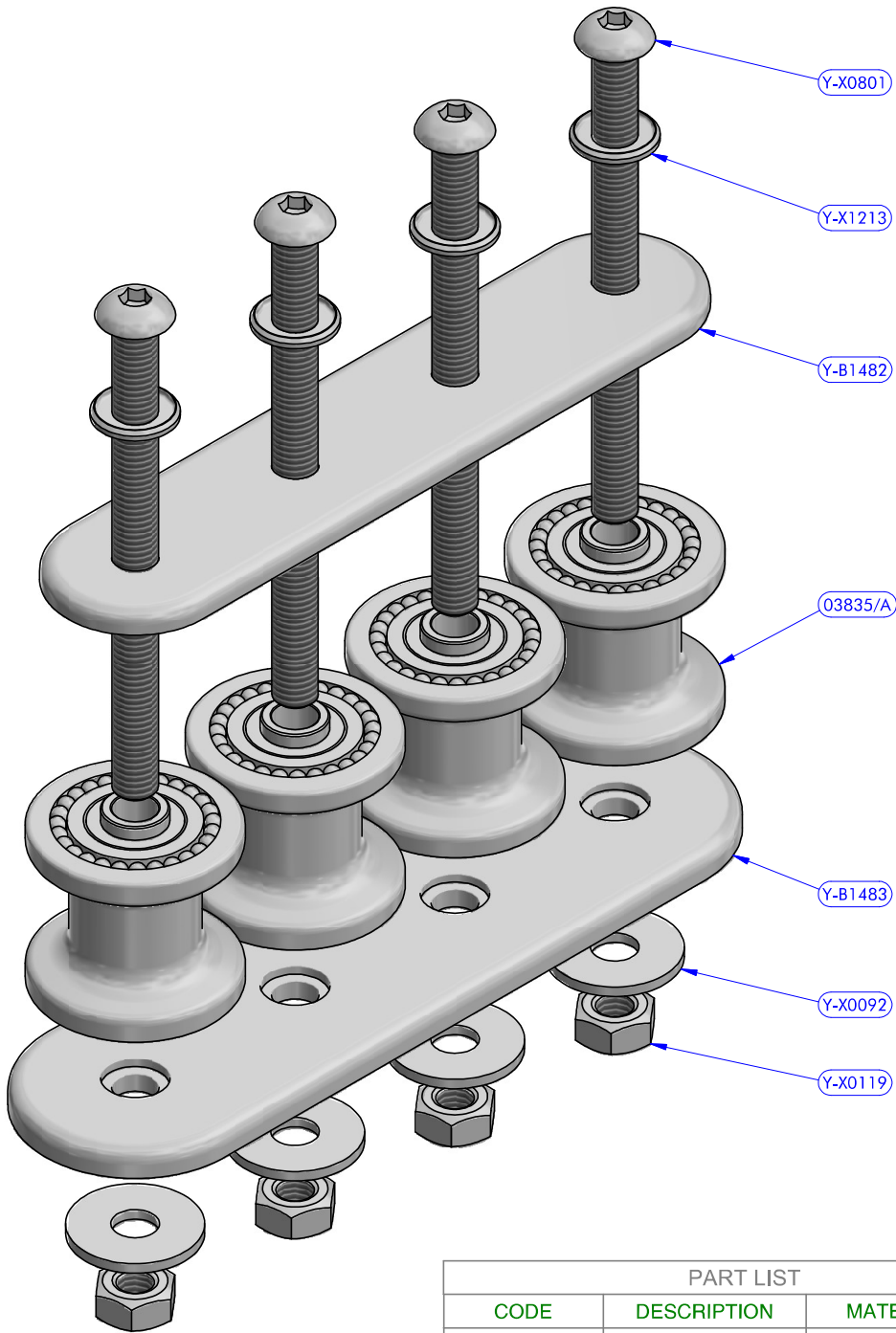
Sheave assy code 03835/A
