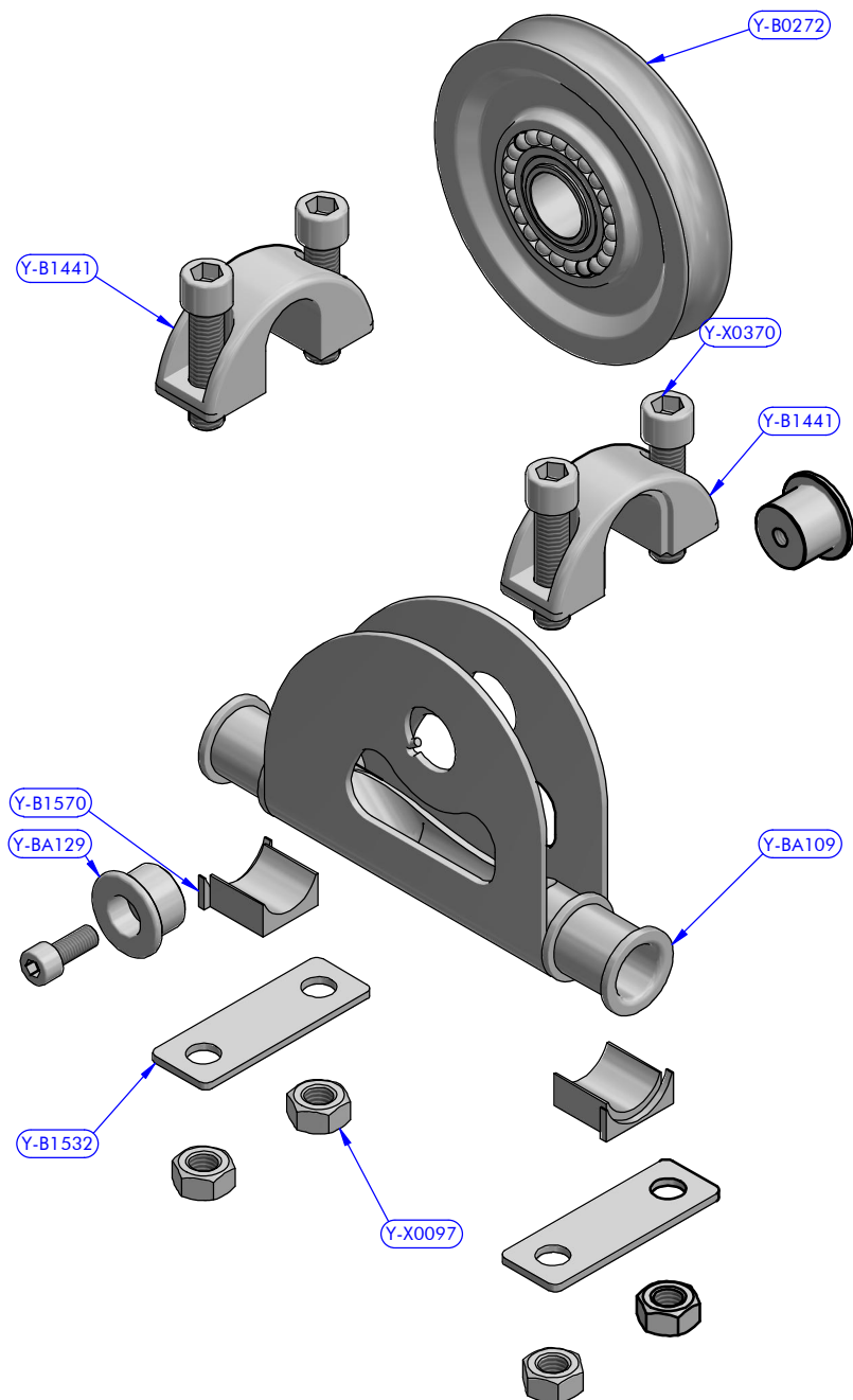
PART LIST 816.120
