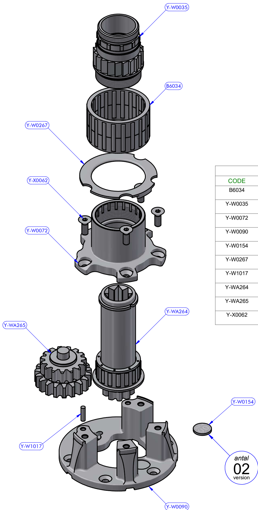
Y-WA267 Base + Gears assy XT30
