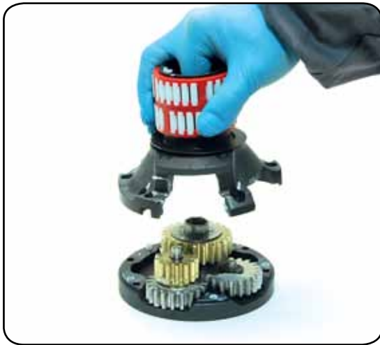
8. Remove the drum support n°14 Important: washer n°11 may remain inside the drum support!
