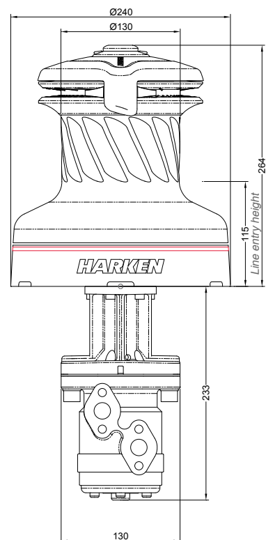
Hydraulic motor
